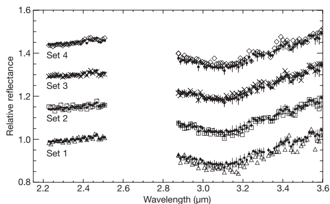
Figure 1 | Rotationally resolved near-infrared reflectance spectra of 24 Themis. The shape and wavelength of the 3.1- \mu\text{m} absorption in this asteroid is interpreted here and in the companion Letter 7 as being due to water ice as opposed to hydrated minerals. There are also absorptions in all our spectra between 3.3 and 3.6 \mu\text{m} that are closely matched by organic compounds 22 . To facilitate searching for possible rotational variation, we grouped the spectra into four separate time intervals, which are plotted in this figure (open symbols and crosses) along with the mean of all our reflectance spectra (solid dots). To plot the reflectance spectrum, we remove the solar spectrum and any thermal emission; at the longest wavelength, 3.6 \mu\text{m} , the subtracted thermal contribution was approximately 20%. The spectra have been normalized at 2.4 \mu\text{m} and for clarity each set is offset from the previous one by 0.15 in relative reflectance. The uncertainties are only plotted for the mean spectrum; error bars correspond to 1 s.d. and the spectral resolution ( \lambda/\Delta\lambda ; \lambda , wavelength) is ~100. We omit the spectral region from 2.45 to 2.83 \mu\text{m} because the Earth's atmosphere is essentially opaque at these wavelengths. We note that the ice and organics absorption bands, at 3.1 \mu\text{m} and between 3.3 and 3.6 \mu\text{m} , preserve their shape and depth throughout the rotation of the asteroid; that is, there is not a significant deviation from the mean in any of the four spectral sets. Hence, the ice and organics are widespread on the surface of this asteroid.
